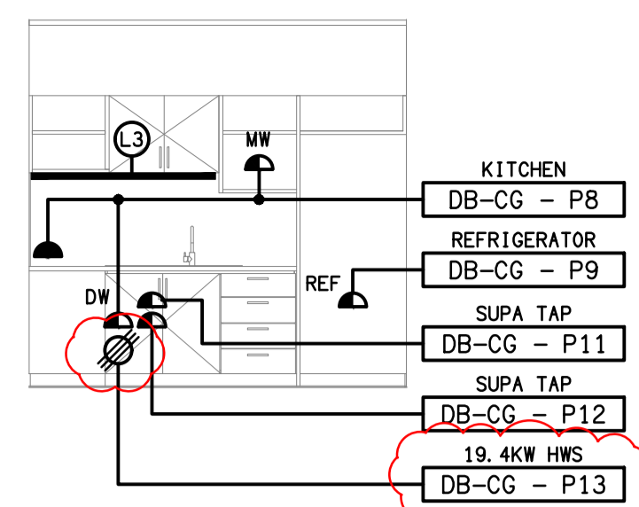
DETAIL A ENTRY KITCHENETTE ELEVATION NOT TO SCALE
